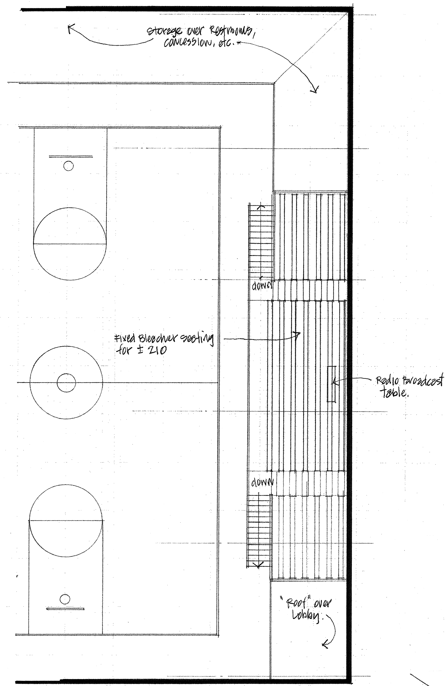
Upper Gymnasium/Bleacher Plan. 1/8" = 1'-0"
