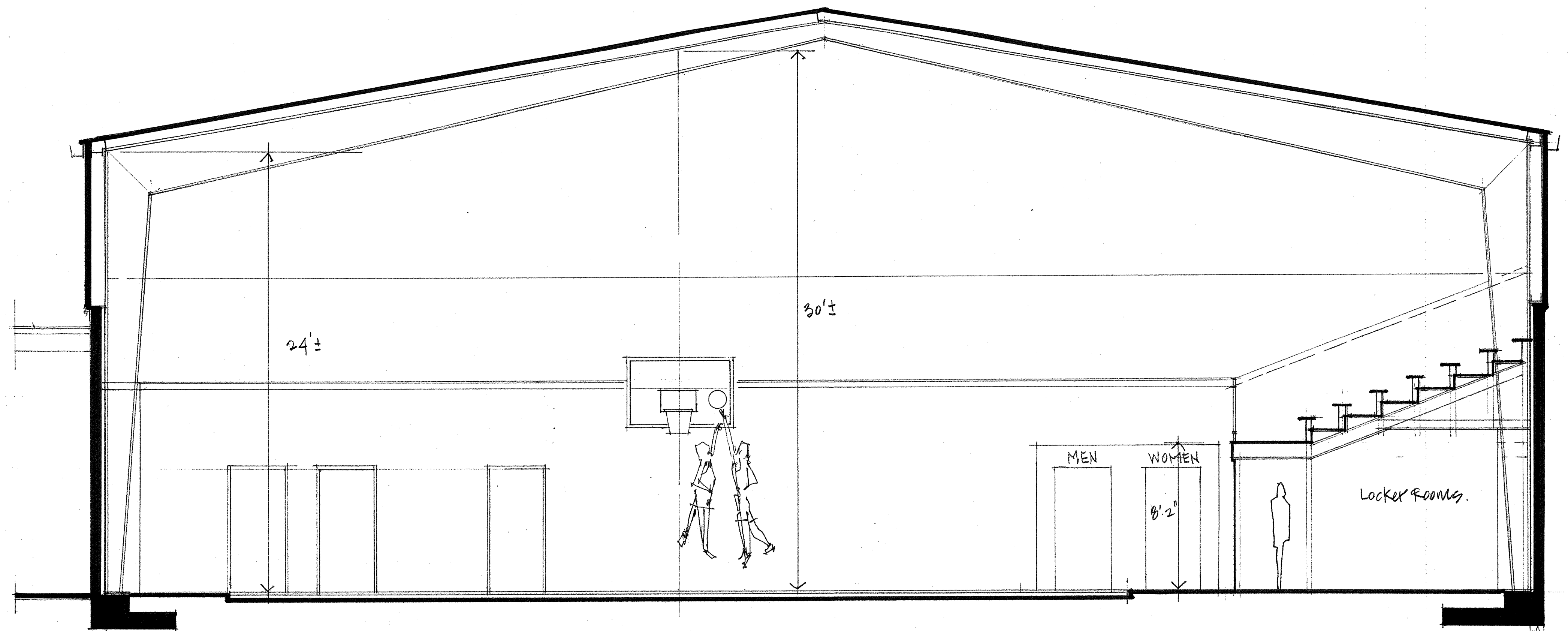
Section thru Gymnasium. 1/8" = 1'-0"
